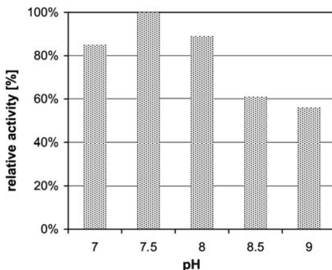
Figure 1. Relative specific activity of E. coli [pQR239] cells at various pH values (measured against racemic bicyclo[3.2.0]hept-2-en-6-one).
