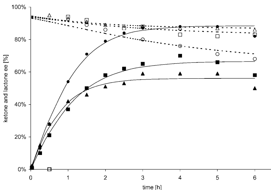
Figure 5. Analytical scale DKR of rac -1: Experimental and simulated effect of Lewatit MP62 on ketone and lactone ees. Experimental (symbol) and simulated (line) ketone (empty symbol) and lactone (black symbol) ees. No resin: ○ and ●; Lewatit MP62 4 meq L -1 : □ and ■; 8 meq L -1 : △ and ▲ (others conditions: 0.3 g L -1 of 1 , pH 7.5, 37 °C).
