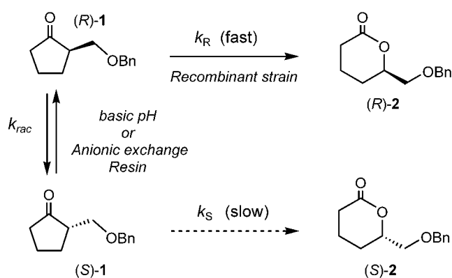
Scheme 1. DKR of rac -1.
