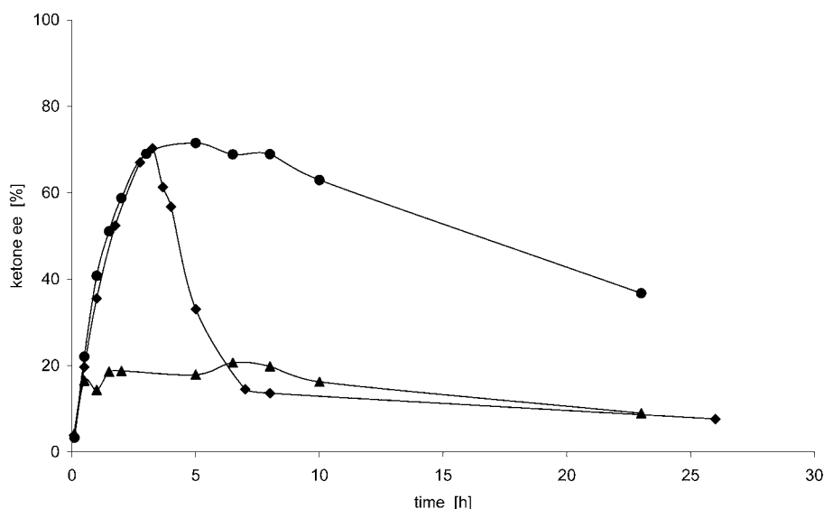
Figure 4. Analytical scale DKR of rac -1. Effect of Lewatit MP62 on unreacted ketone ees. No resin: ●; addition of resin (24.5 meq L -1 ) at time 0: ▲; after 3.5 h: ◆ (other conditions: 1 g L -1 of rac -1, pH 7.5, 30 °C).
