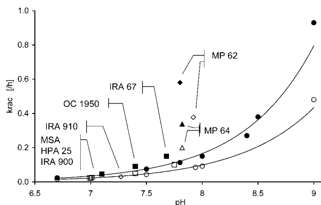
Figure 2. Racemisation constants ( k_{rac} ) with respect to pH. Empty symbols: racemisation at 30 °C; filled symbols: racemisation at 37 °C; full lines, black circle and empty circle: pH-dependent racemisation (addition of KOH to the culture medium); other single symbols: racemisation with various anionic resins (12.5 meq L -1 ), ♦ and ◇ Lewatit MP62, ▲ and △ Lewatit MP64, ■ and □ other resins.
