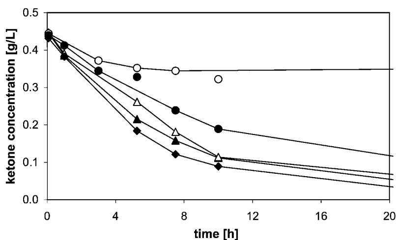
Figure 3. Determination of the inhibitory level of lactone 2 . Time dependent concentration of rac - 1 in the presence of various initial concentrations of rac - 2 : \blacklozenge 0, \blacktriangle 0.5, \triangle 0.7, \bullet 1.0 and \circ 1.5 \text{ g L}^{-1} (other conditions: 30^\circ\text{C} , pH 7, 0.5 \text{ g L}^{-1} of rac - 1 ).
